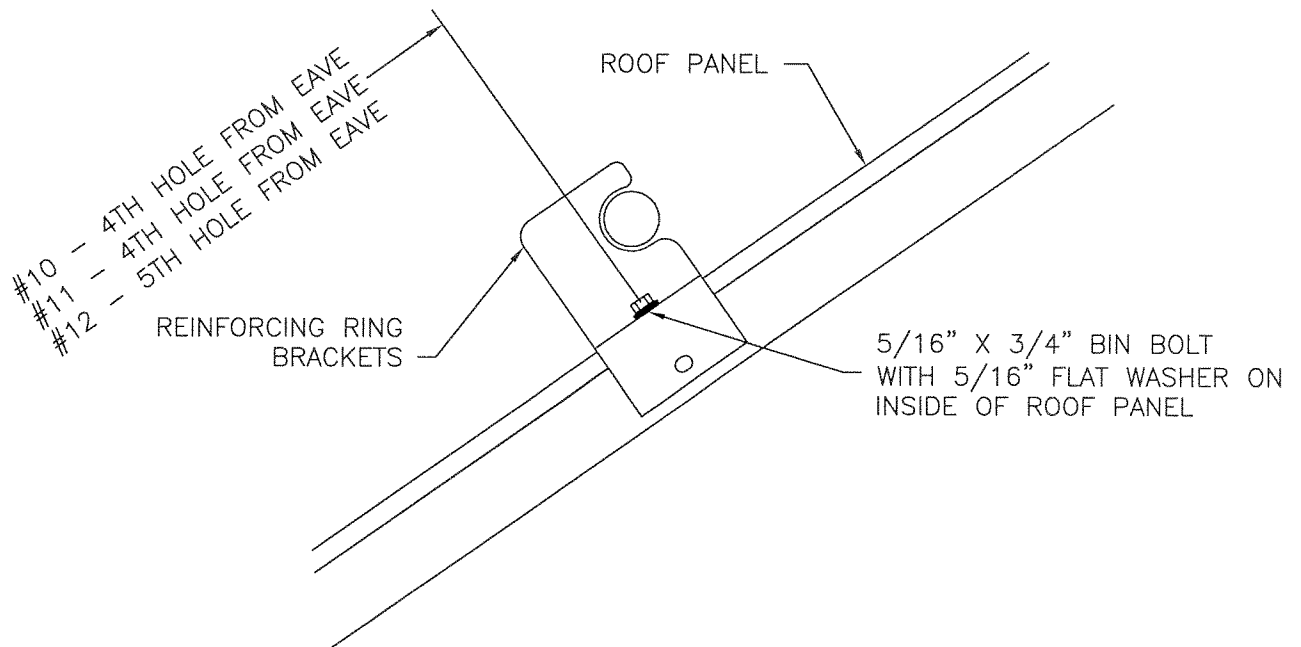
Reinforcing Ring Installation Detail for #10, #11, and #12 Roofs
