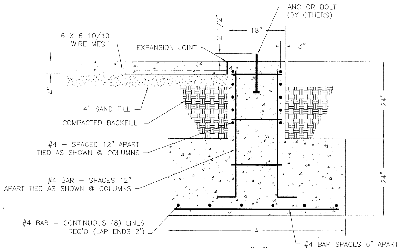
FOUNDATION TYPE "E"
