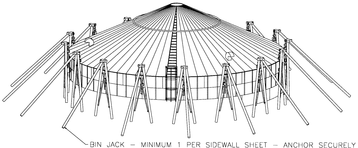
BIN JACK — MINIMUM 1 PER SIDEWALL SHEET — ANCHOR SECURELY
