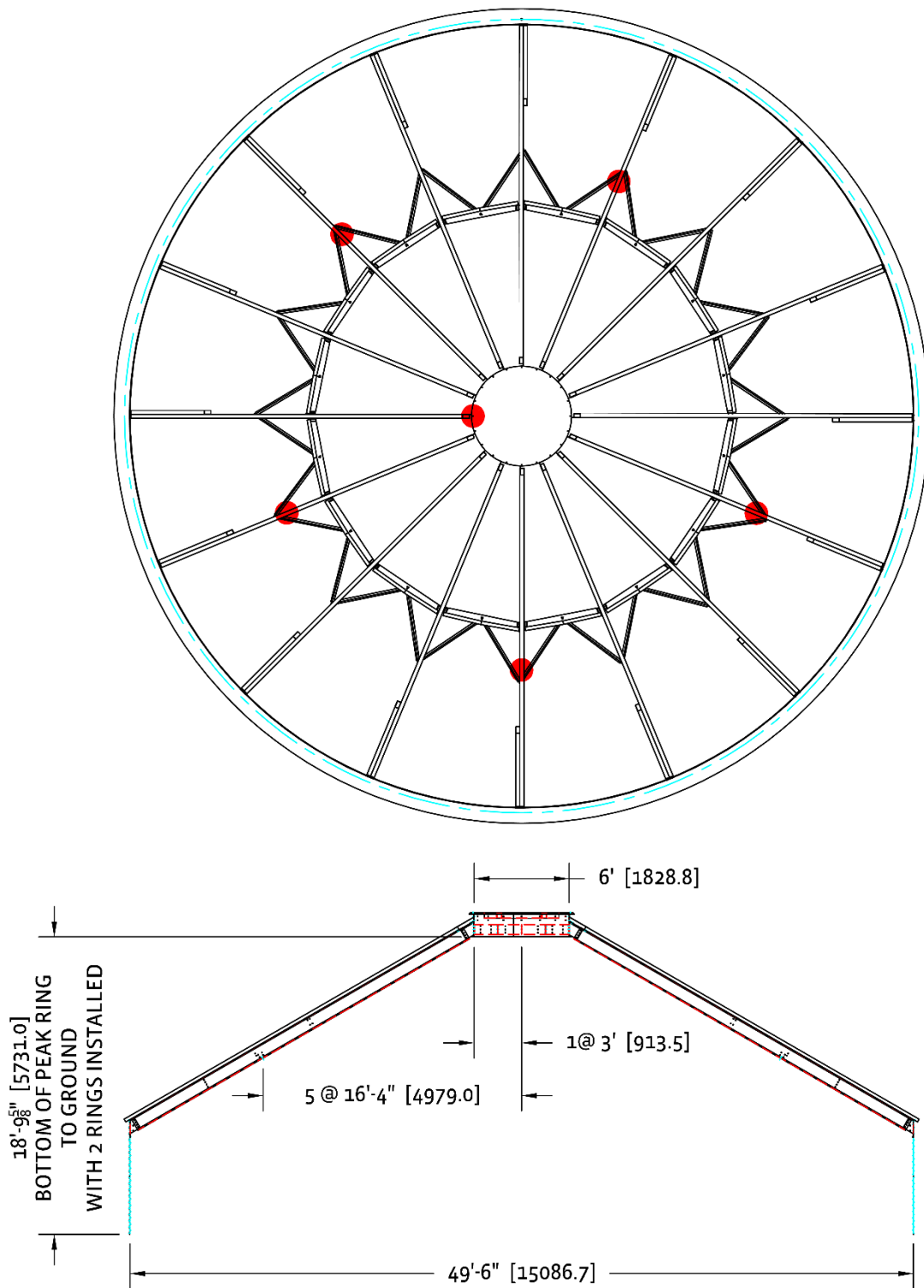
CB16 (49'-6") TEMP. CABLE LAYOUT (15 RINGS AND SHORTER)
