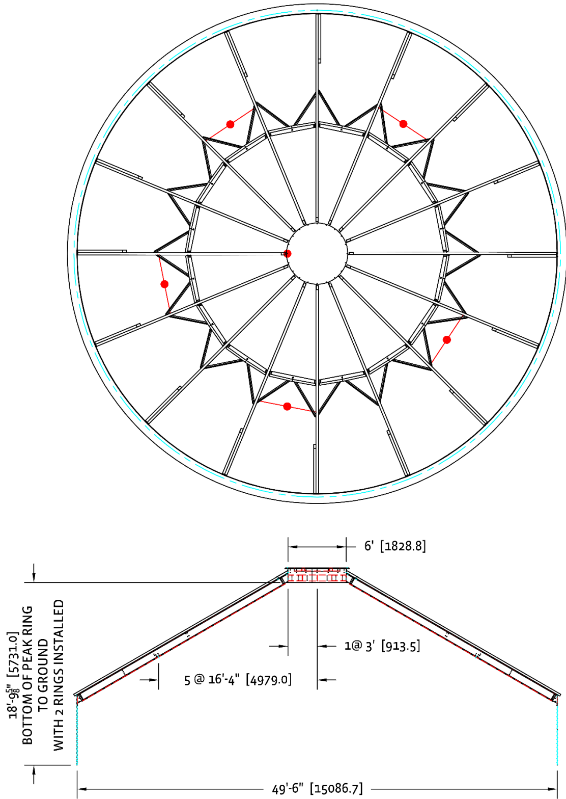
CB16 (49'-6") TEMP. CABLE LAYOUT (16 RINGS AND TALLER)
