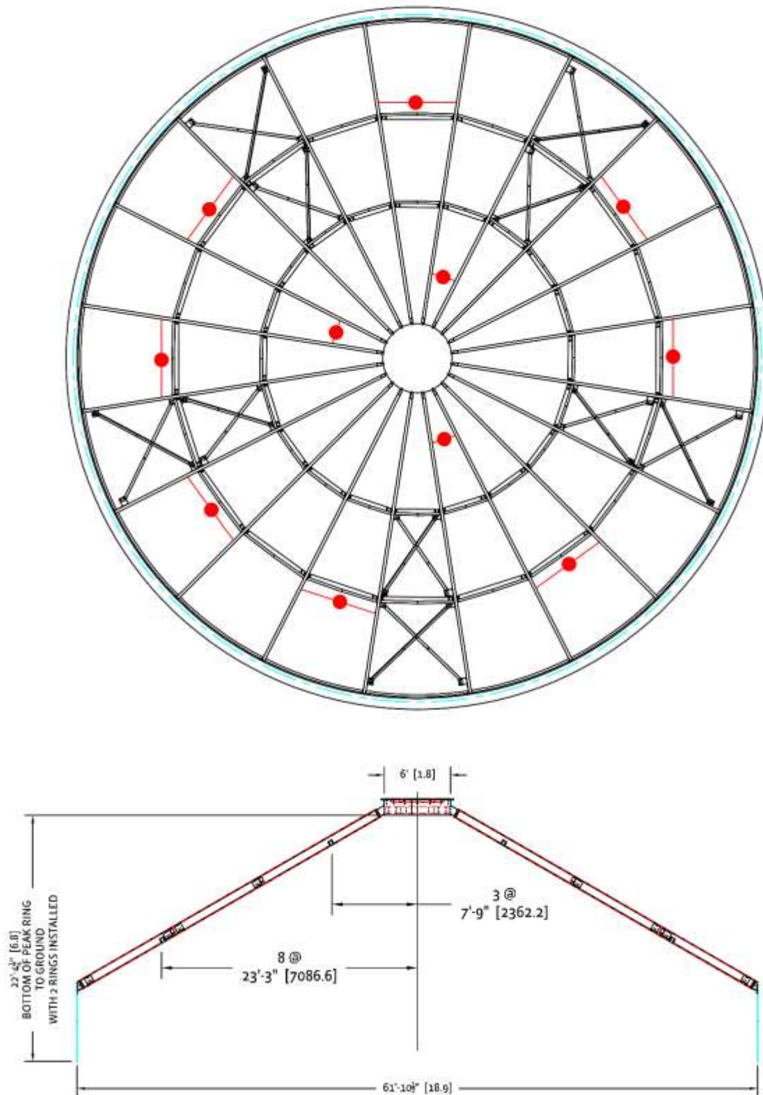
CB20 (61'-10") TEMP. CABLE LAYOUT (16 RINGS AND TALLER)
