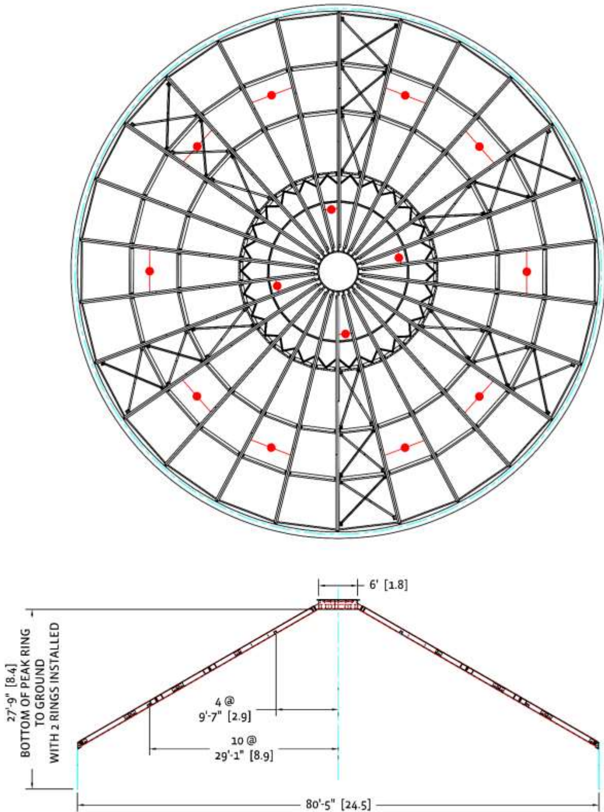
CB26 (80'-5") TEMP. CABLE LAYOUT (16 RINGS AND TALLER)
