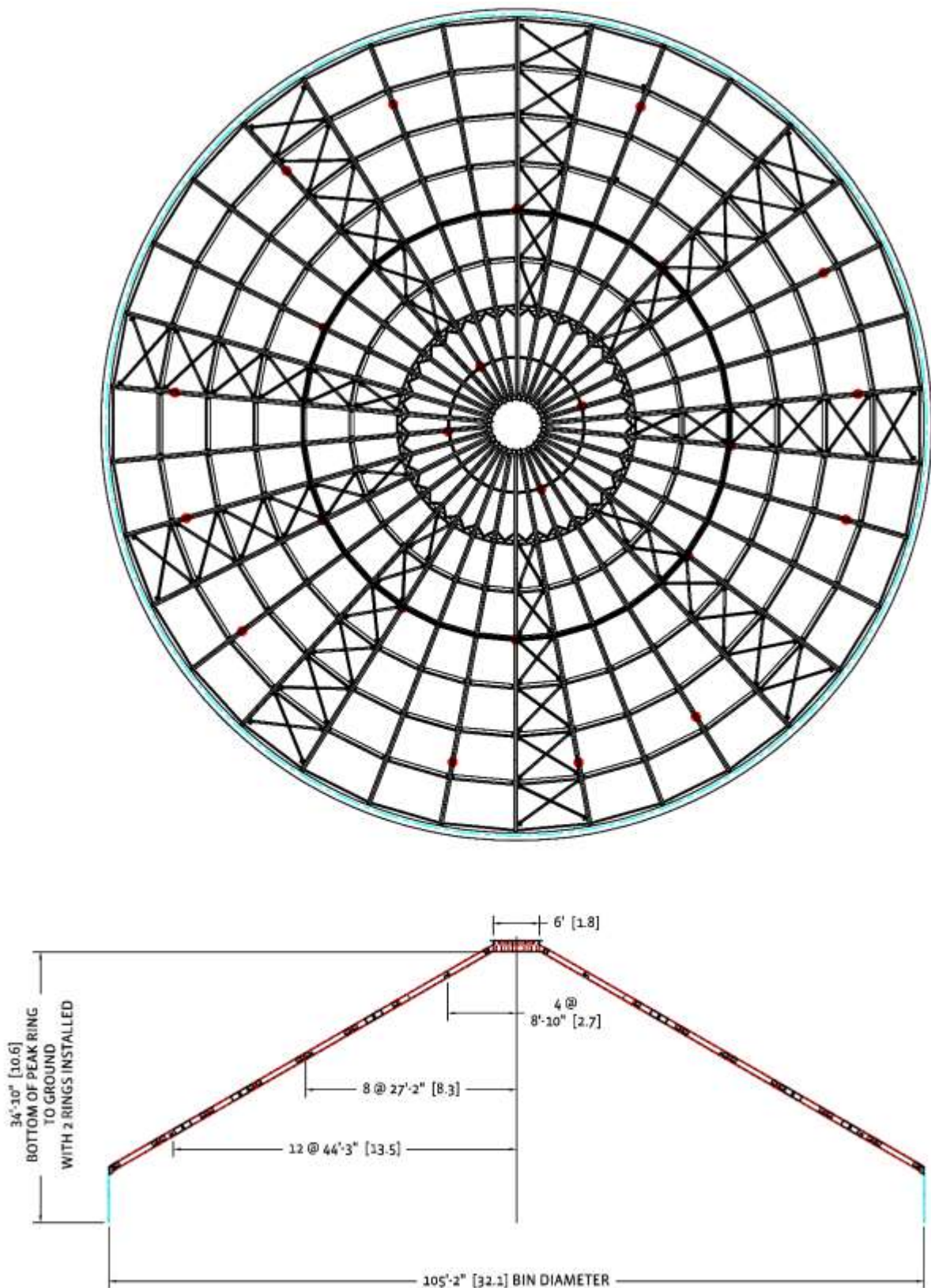
CB34 (105'-2") TEMP. CABLE LAYOUT (15 RINGS AND SHORTER)
