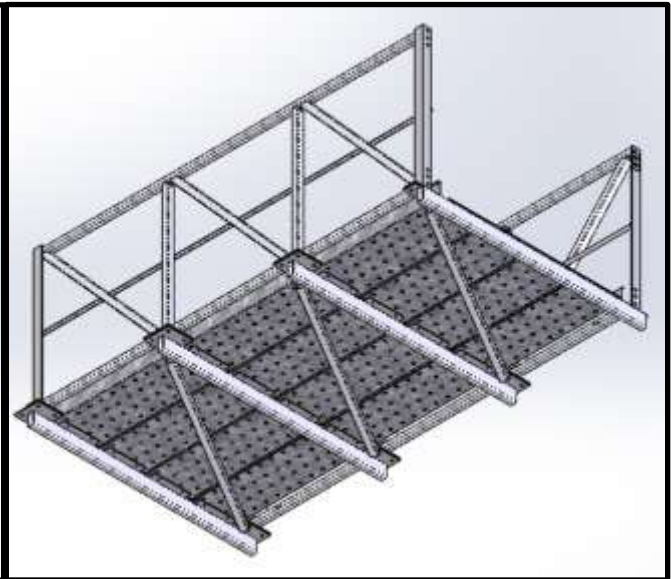
#2-30" Conveyor Mounting Catwalk with Full Floor Walkway Bottom View
