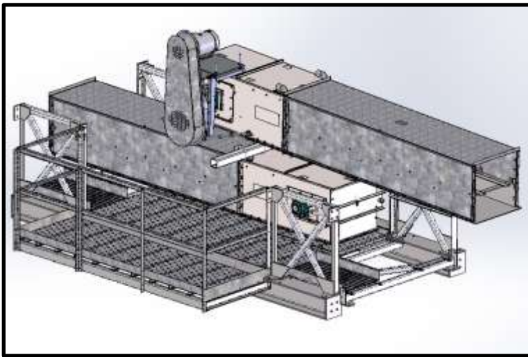
Continuous Walkaround with Piggy-Back Conveyors.
