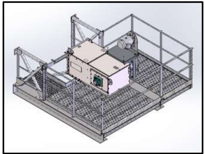
Peak End Walkaround with Conveyor Head Section.
